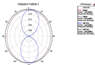
Fig 6: 2D Pattern of Gain Total for \phi = 0 and \phi = 90 Degrees
