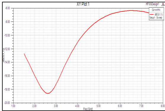
Fig. 2 S-parameter plots for Return Loss v/s Frequency
