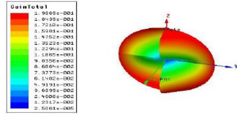
Fig 7: 3D Pattern of gain Total for \phi = 0 and \phi = 90 Degrees
